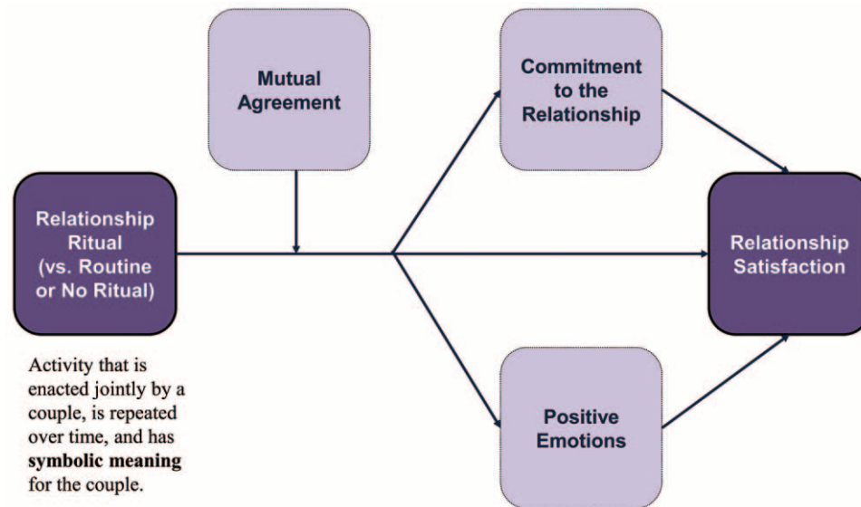
Figure 1. Theoretical framework.
